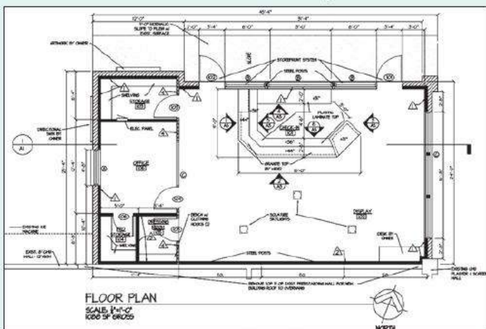
Updated Floor Plan
